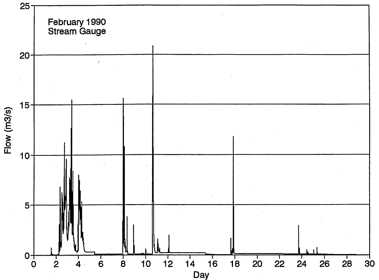
FIGURE 5 STREAMFLOW AND PLUVIOGRAPH DATA FEBRUARY 1990
