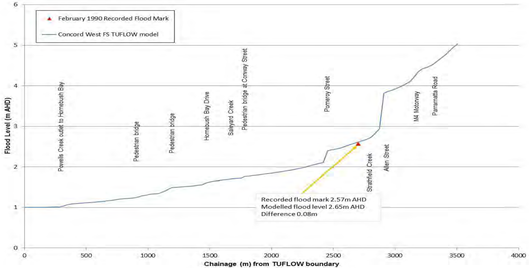
Figure 5-1 Powells Creek mainstream flood profile, 10 February 1990 calibration event
